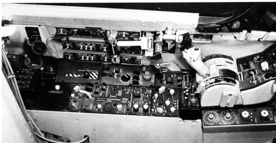
Left console of F-105F forward cockpit. ("D" model is similar) (Republic)
