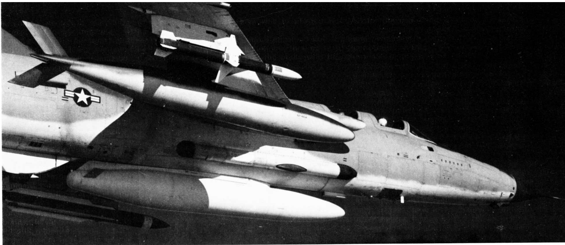
F-105F, fitted with QRC (Quick Reaction Contract) - 380 ECM blisters, shown during flight testing of the F-105G modifications. It carries practice AGM-45 "Shrike" missile on right pylon, and AGM-78B Standard ARM on left pylon. (USAF)
