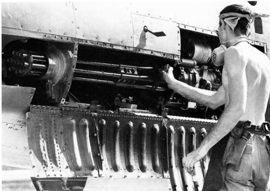
Armament specialist services the M-61 20mm cannon. Angle of attack indicator is visible just above cannon. (D.M. Weaver via Jim Farmer)
